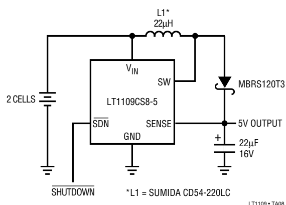
3V to 5V Converter with Shutdown
