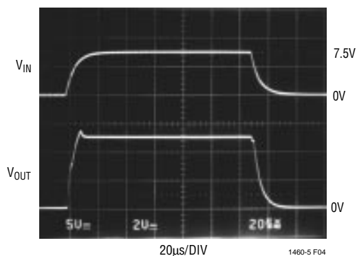
Figure 5. C IN = 0.1µF
