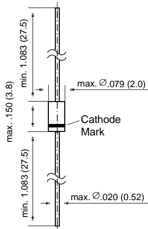
DO-35
