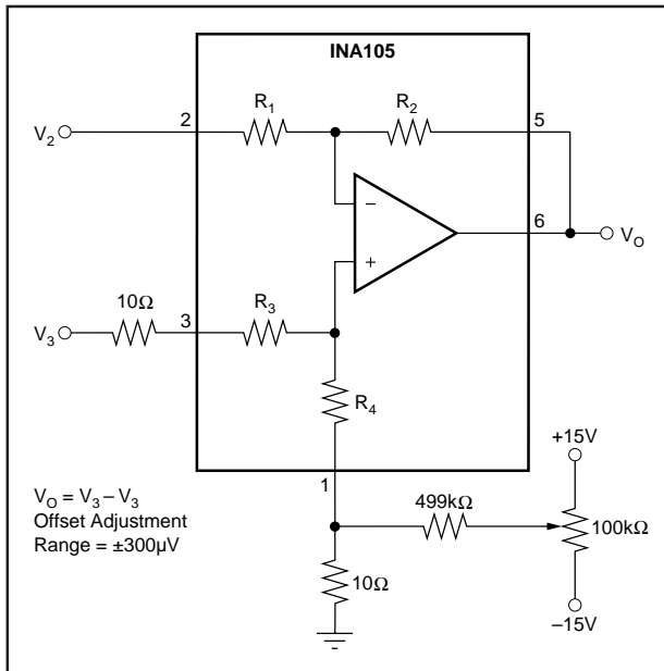
FIGURE 2. Offset Adjustment.
