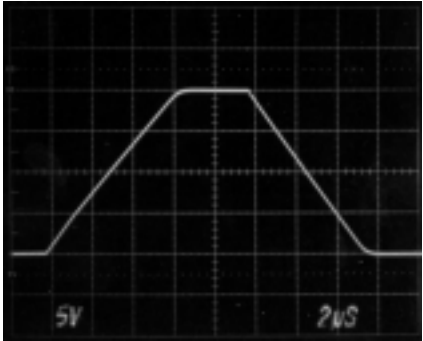
STEP RESPONSE
