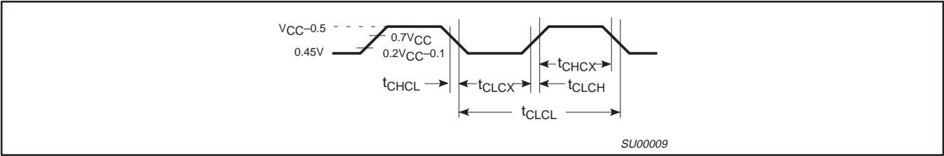
Figure 19. Clock Signal Waveform for I_{CC} Tests in Active and Idle Modes t_{CLCH} = t_{CHCL} = 5ns
