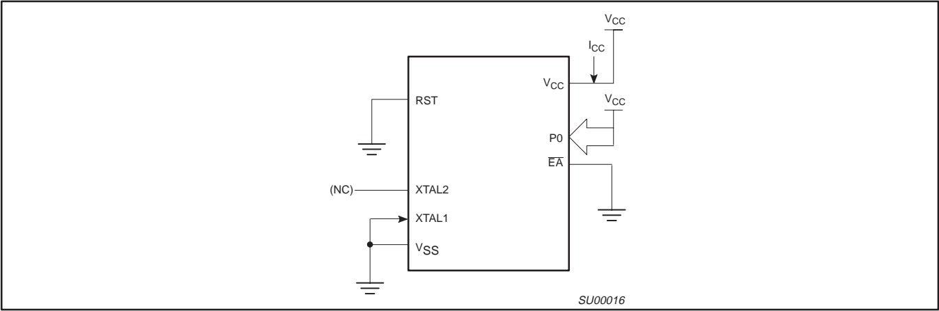
Figure 20. I_{CC} Test Condition, Power Down Mode All other pins are disconnected. V_{CC} = 2V to 5.5V
