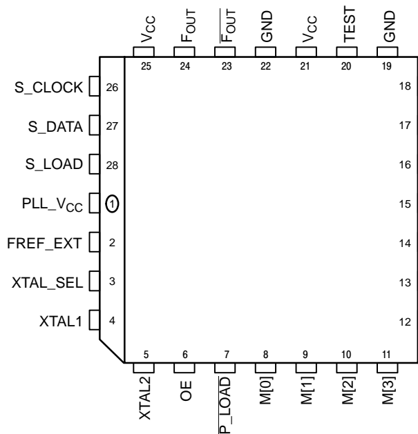
Figure 2. 28-Lead PLCC (Top View)
