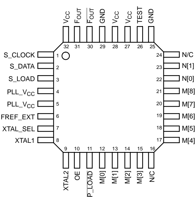
Figure 3. 32-Lead LQFP (Top View)
