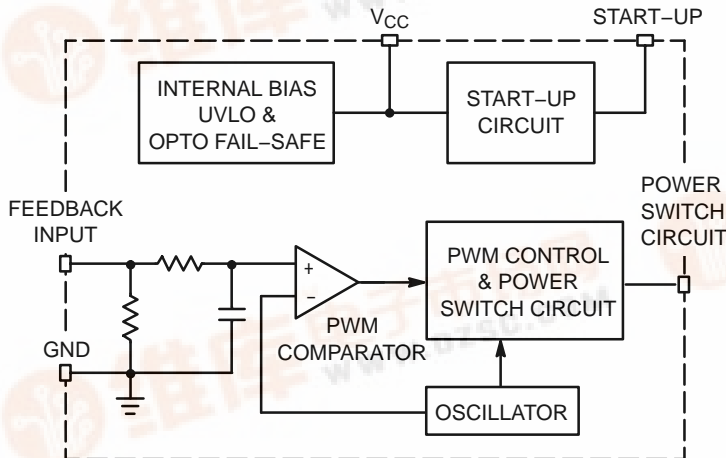
Figure 1. Simplified Block Diagram
