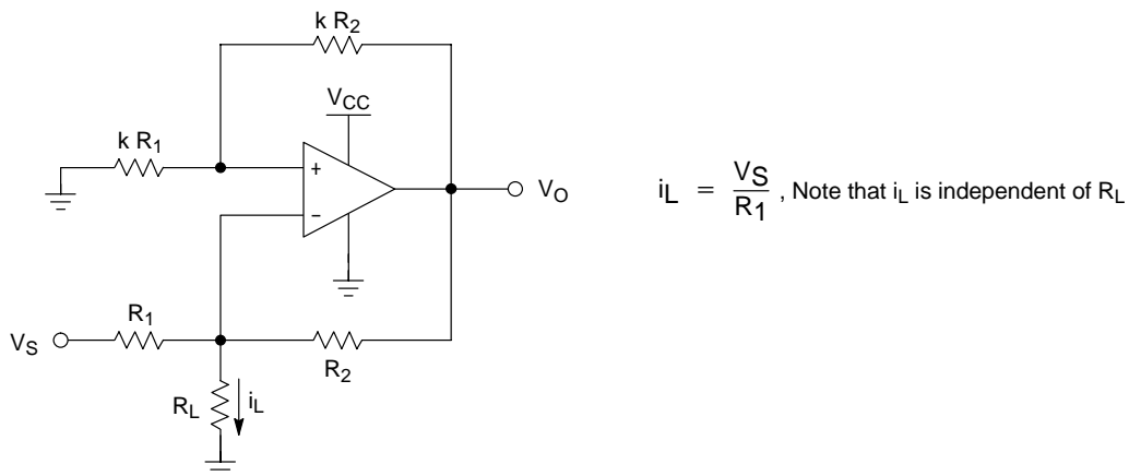
Figure 40. Current Source
