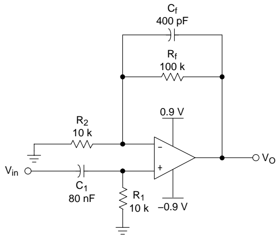
Figure 37. Voice Band Filter
