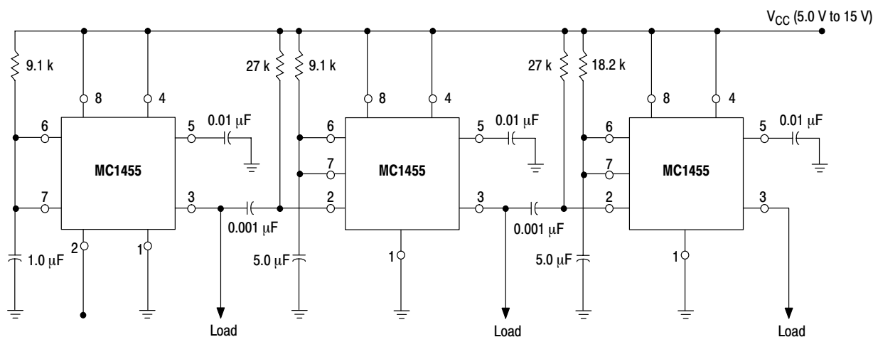
Figure 26. Sequential Timer
