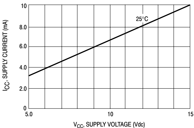
Figure 5. Supply Current
