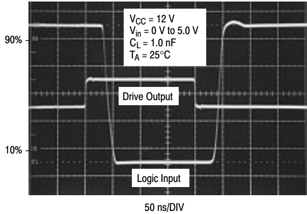
Figure 8. Propagation Delay
