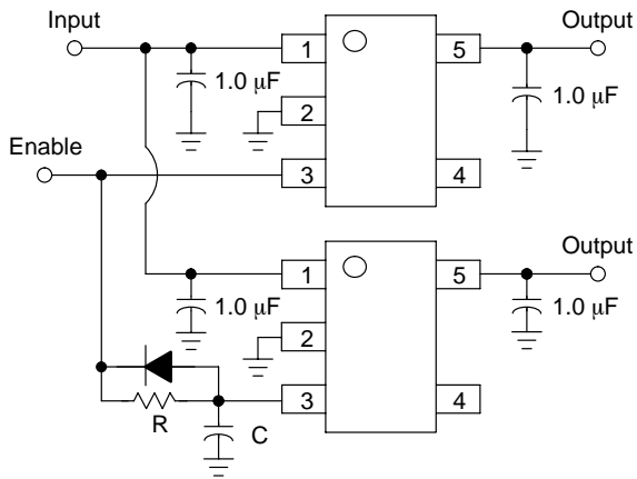
Figure 23. Delayed Turn-on
