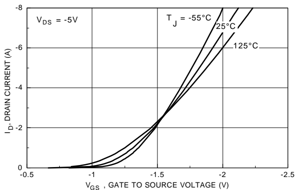
Figure 5. Transfer Characteristics.
