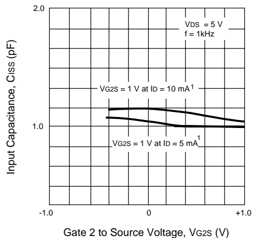
INPUT CAPACITANCE vs. GATE 2 TO SOURCE VOLTAGE
