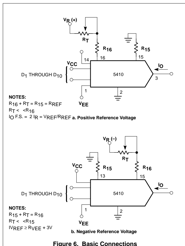
Figure 6. Basic Connections
