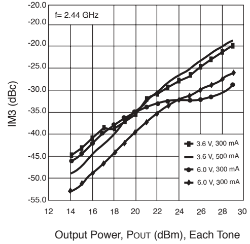
IM3 vs. OUTPUT POWER
