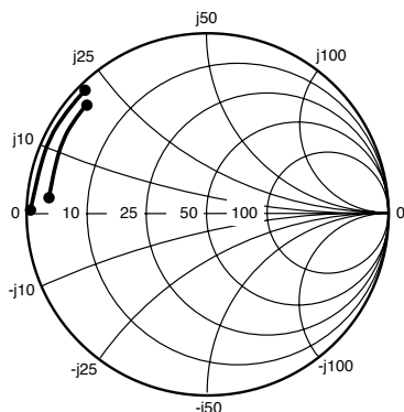
Coordinates in Ohms Frequency in GHz V D = 3.5 V, I D = 150 mA
