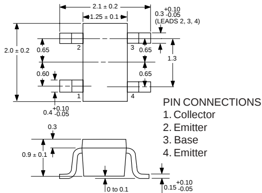
PACKAGE OUTLINE 18
