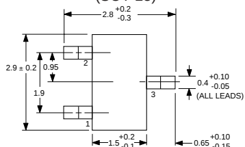
PACKAGE OUTLINE 33
