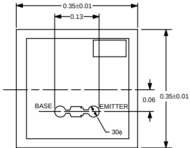
PACKAGE OUTLINE 18
