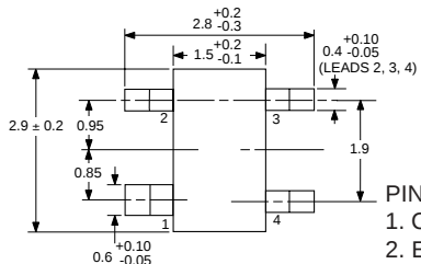
PACKAGE OUTLINE 39
