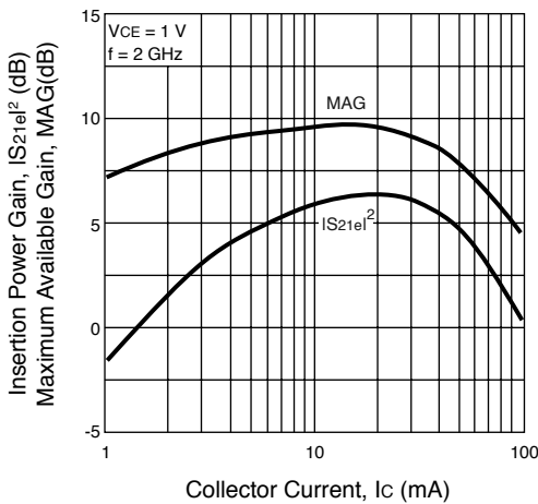
INSERTION POWER GAIN and MAG vs. COLLECTOR CURRENT
