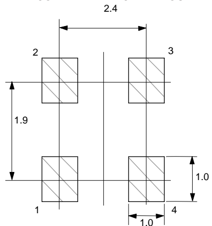
PACKAGE OUTLINE 39R RECOMMENDED P.C.B. LAYOUT
