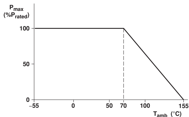
Maximum dissipation ( P_{\max} ) in percentage of rated power as a function of the ambient temperature ( T_{\text{amb}} ).
