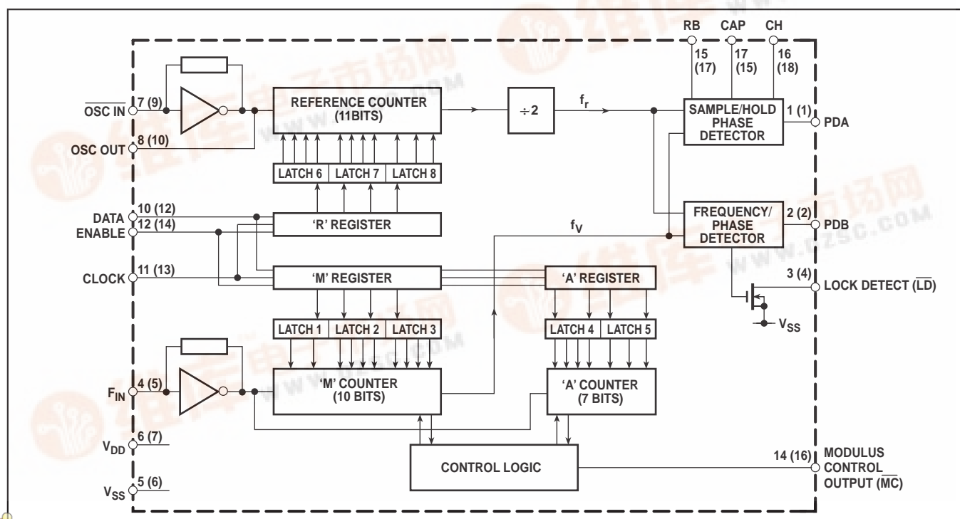
Fig.2 Block diagram (MP pinout shown in parentheses)
