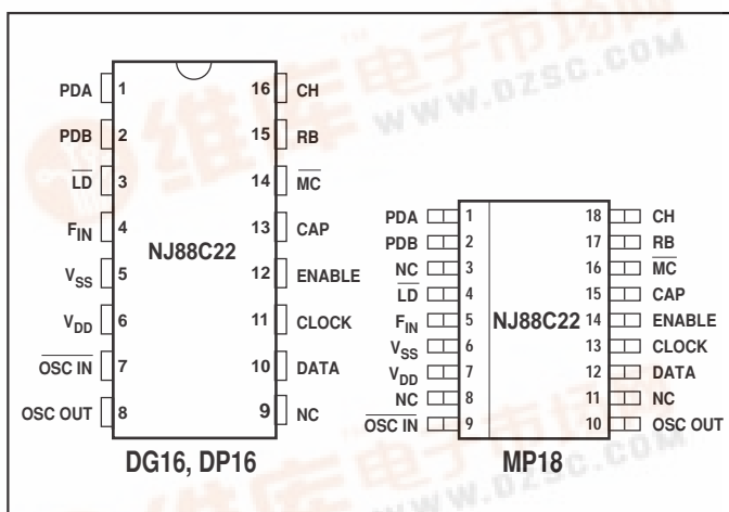
Fig.1 Pin connections - top view (not to scale)
