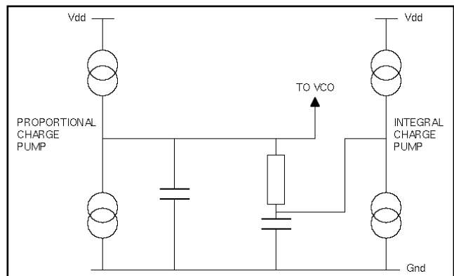
Fig.5 Loop filter using both charge pumps
