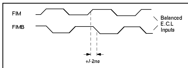
Fig.4 Maximum input skew
