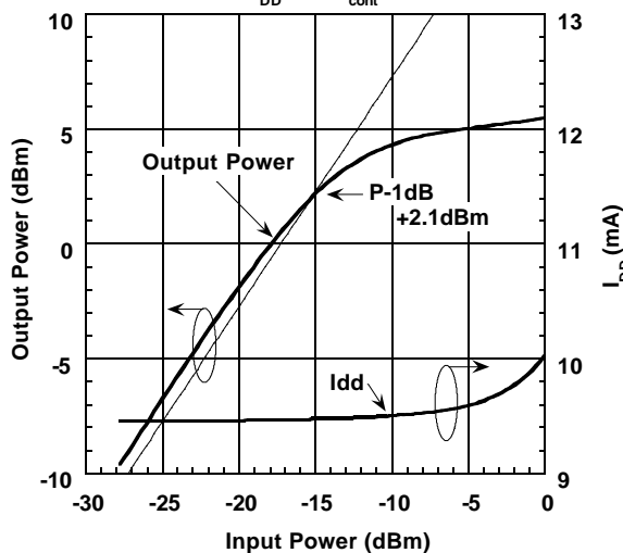
OUTPUT POWER, I_{DD} vs. INPUT POWER ( V_{DD}=3V, V_{cont}=2V, f=938MHz )
