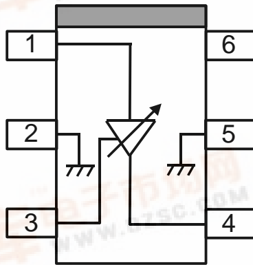
F TYPE (Top View)
