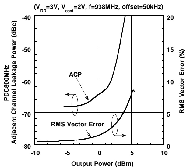
ACP, RMS VECTOR ERROR vs. OUTPUT POWER ( V_{DD}=3V, V_{cont}=2V, f=938MHz, offset=50kHz )
