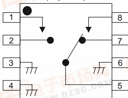
R TYPE (Top View)
