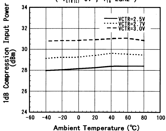
P-1dB vs. Temperature ( V_{CTR(LI)}=0V , f_{in}=2GHz )
