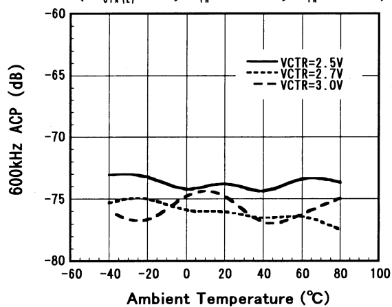
600kHz ACP vs. Temperature ( V_{CTR(LI)}=0V , f_{in}=1.9GHz , P_{in}=22dBm )
