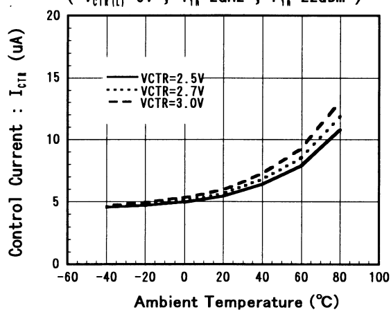
Control Current vs. Temperature ( V_{CTR(LI)}=0V , f_{in}=2GHz , P_{in}=22dBm )
