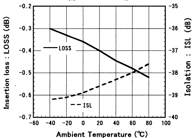
Loss/Isolation vs. Temperature ( V_{CTR}=0V/2.7V , f_{in}=2GHz )
