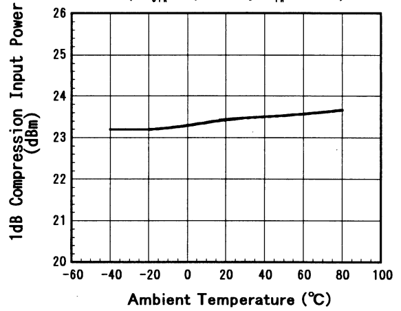
P-1dB vs. Temperature ( V_{CT1}=0V/2.7V , f_{i1}=2GHz )
