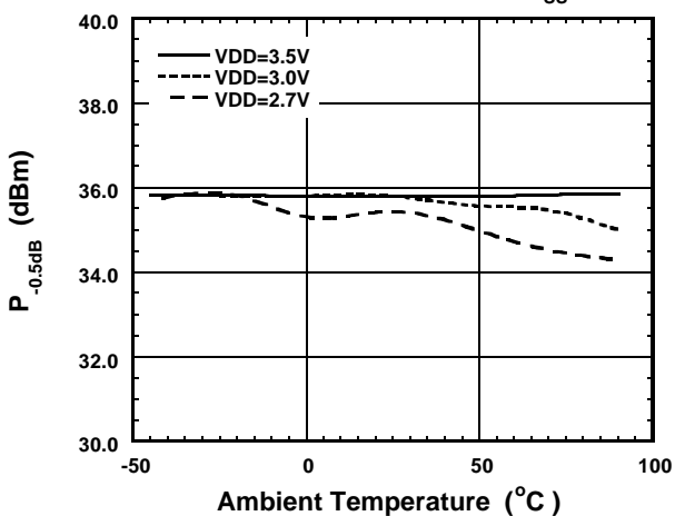
P_{-0.5\text{dB}} vs. Ambient Temperature vs. V_{DD} (Tx-Ant1, f=940\text{MHz} , V_{SS}=-2.5\text{V} )
