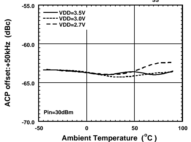
ACP(+50kHz) vs. Ambient Temperature vs. V_{DD} (Tx-Ant1, f=940\text{MHz} , V_{SS}=-2.5\text{V} )
