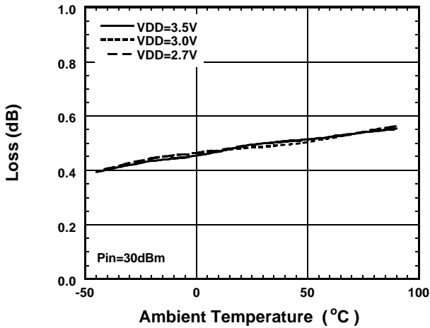
Loss vs. Ambient Temperature vs. V_{DD} (Tx-Ant1, f=940\text{MHz} , V_{SS}=-2.5\text{V} )
