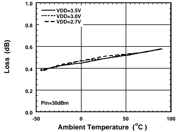
Loss vs. Ambient Temperature vs. V_{DD} (Tx-Ext1, f=940\text{MHz} , V_{SS}=-2.5\text{V} )
