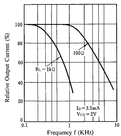
Output Current vs. Frequency ( T_a = 25^\circ\text{C} )
