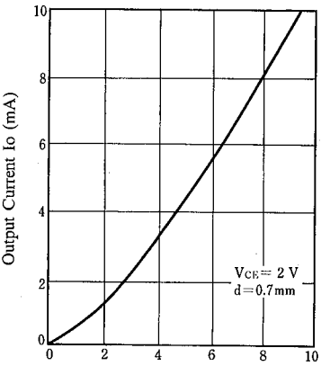
Output Current vs. Forward Current ( T_a=25^{\circ}\text{C} )
