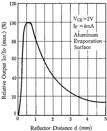
Output Current vs. Distance ( T_a \approx 25^\circ\text{C} )
