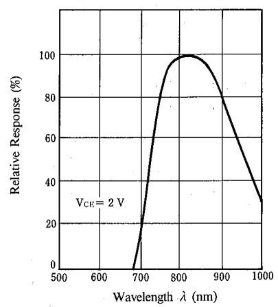
Spectral Response ( T_a = 25^\circ\text{C} )
