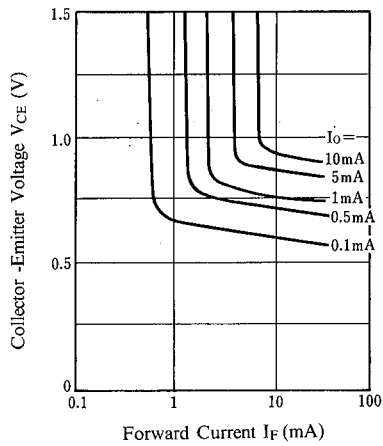
V_{CE} Saturation ( T_a = 25^\circ\text{C} )
