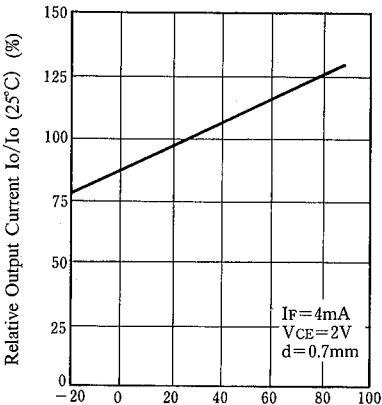
Output Current vs. Temperature
