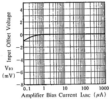
Input Offset Voltage
