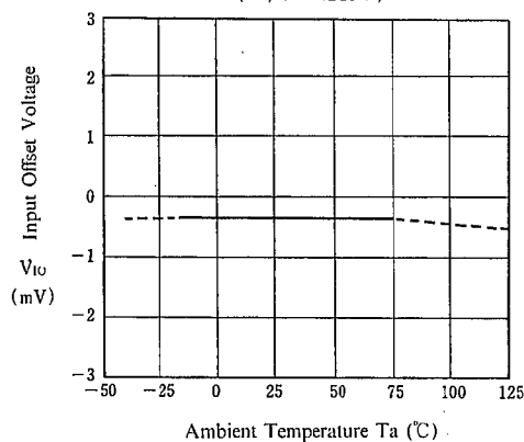
Input Offset Voltage vs. Temperature ( V^+/V^- = \pm 15\text{V} )
