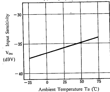
Input Sensitivity vs. Ambient Temperature
