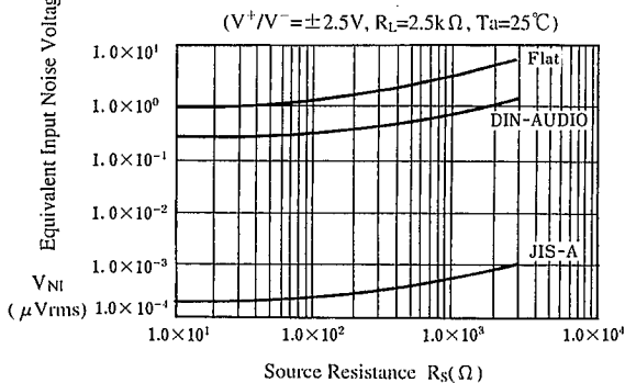
Equivalent Input Noise Voltage vs. Source Resistance
