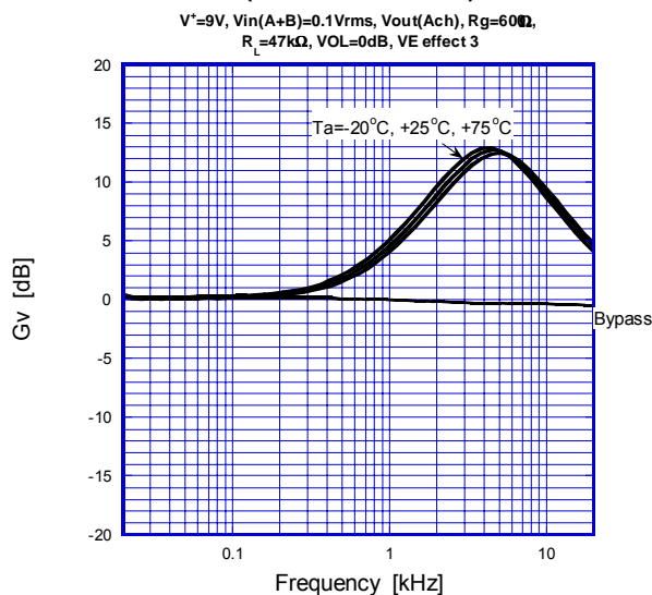
fig.41 Voltage Gain vs Frequency (Voice Enhancement)
