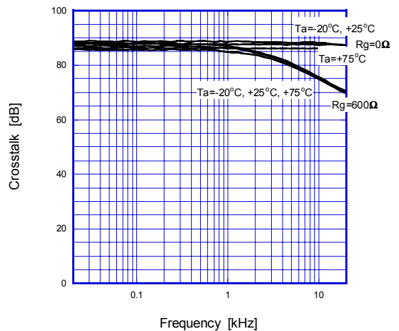
fig.24 Crosstalk vs Frequency
