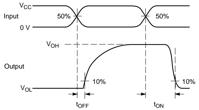
Figure 3. t_{ON}/t_{OFF}
