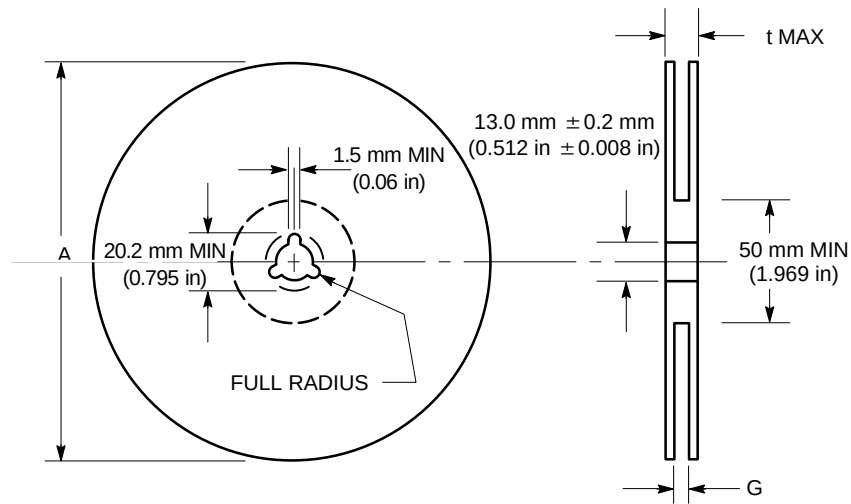
Figure 20. Reel Dimensions
