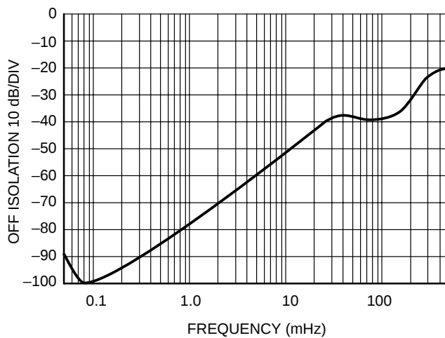
Figure 12. Off Isolation
