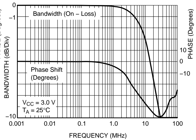
Figure 24. NO Bandwidth and Phase Shift versus Frequency
