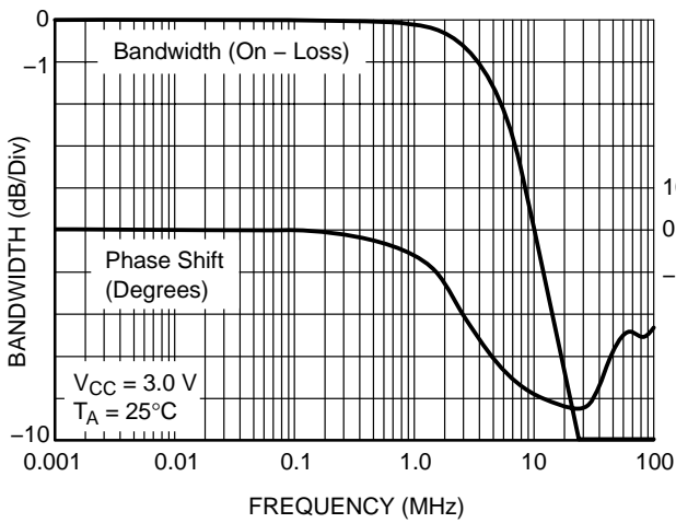
Figure 23. NC Bandwidth and Phase Shift versus Frequency
