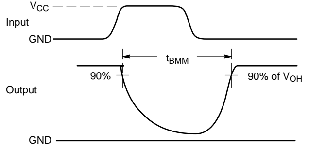
Figure 4. t_{\text{BMM}} (Time Break-Before-Make)
