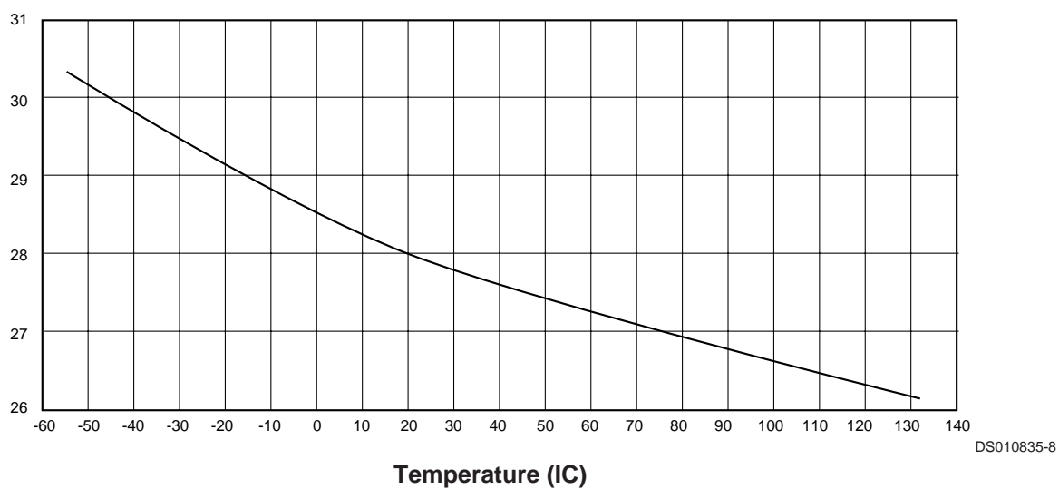
I_{CC} vs. Temperature
