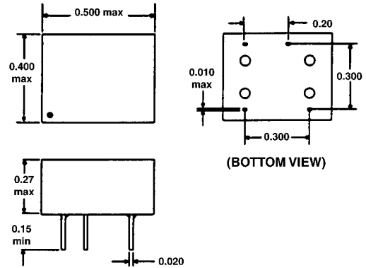
DUAL-IN-LINE PACKAGE
