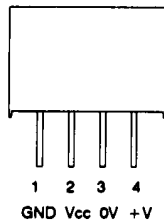
SINGLE-IN-LINE PACKAGE
