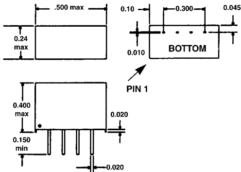
SINGLE-IN-LINE PACKAGE
