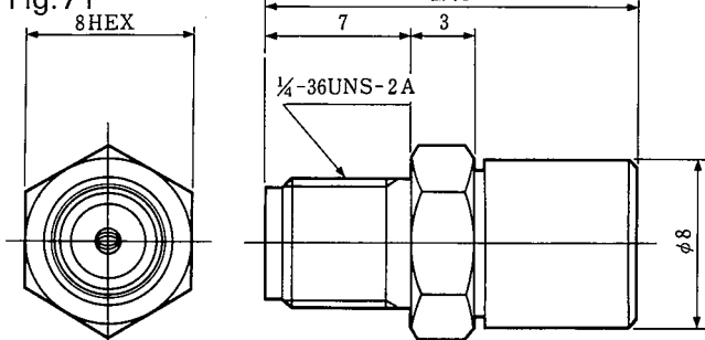
HRMJ-FLJ CL311-0179-3
