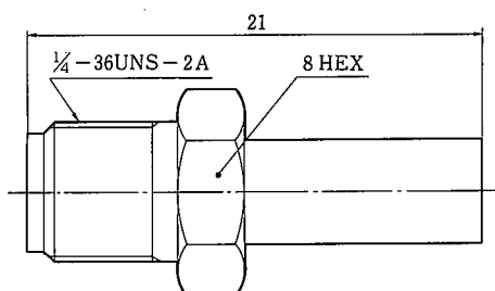
HRMJ-PO51P CL311-0231-1
