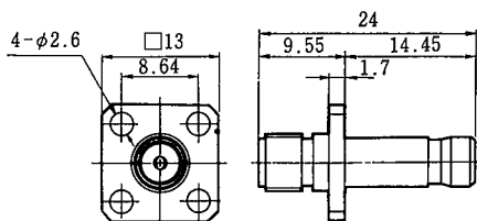
HRMJ-POBJ-PA CL311-0150-1
