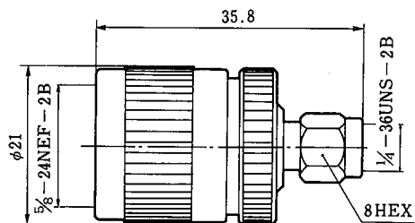
HRM-509 (09) CL311-0093-0-09
