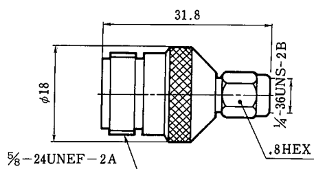
HRM-553S CL311-0121-3
