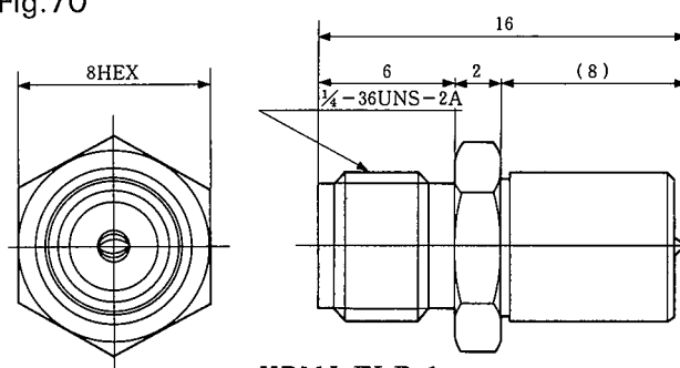
HRMJ-FLP-1 CL311-0195-0
