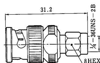
HRM-519 (09) CL311-0101-6-09
