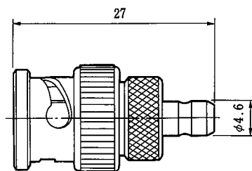
BNCP-MSSJ CL311-0082-3
