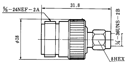
HRM-507 (09) CL311-0091-4-09
