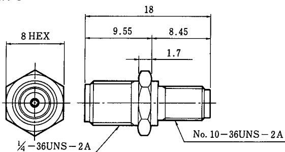
HRMJ-HRMMJ CL311-0220-5
