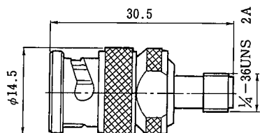
HRM-518(09) CL311-0100-3-09
