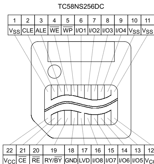
Figure 1. Pinout
