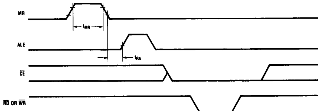
Reset Timing
