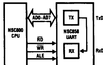
FIGURE 4. Local Loopback
