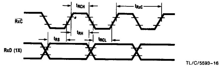
Receiver Timing
