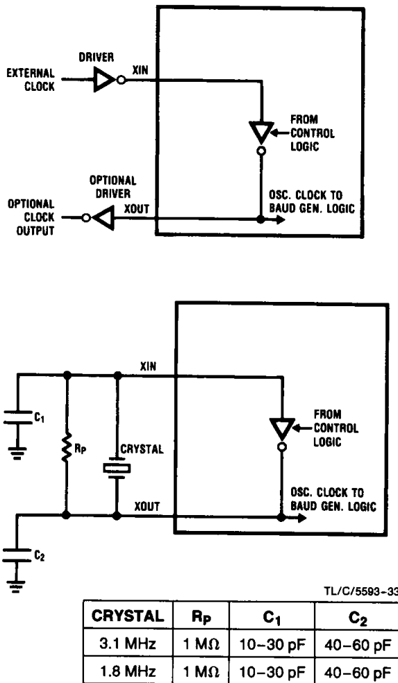
FIGURE 2. Typical Crystal Oscillator Network
