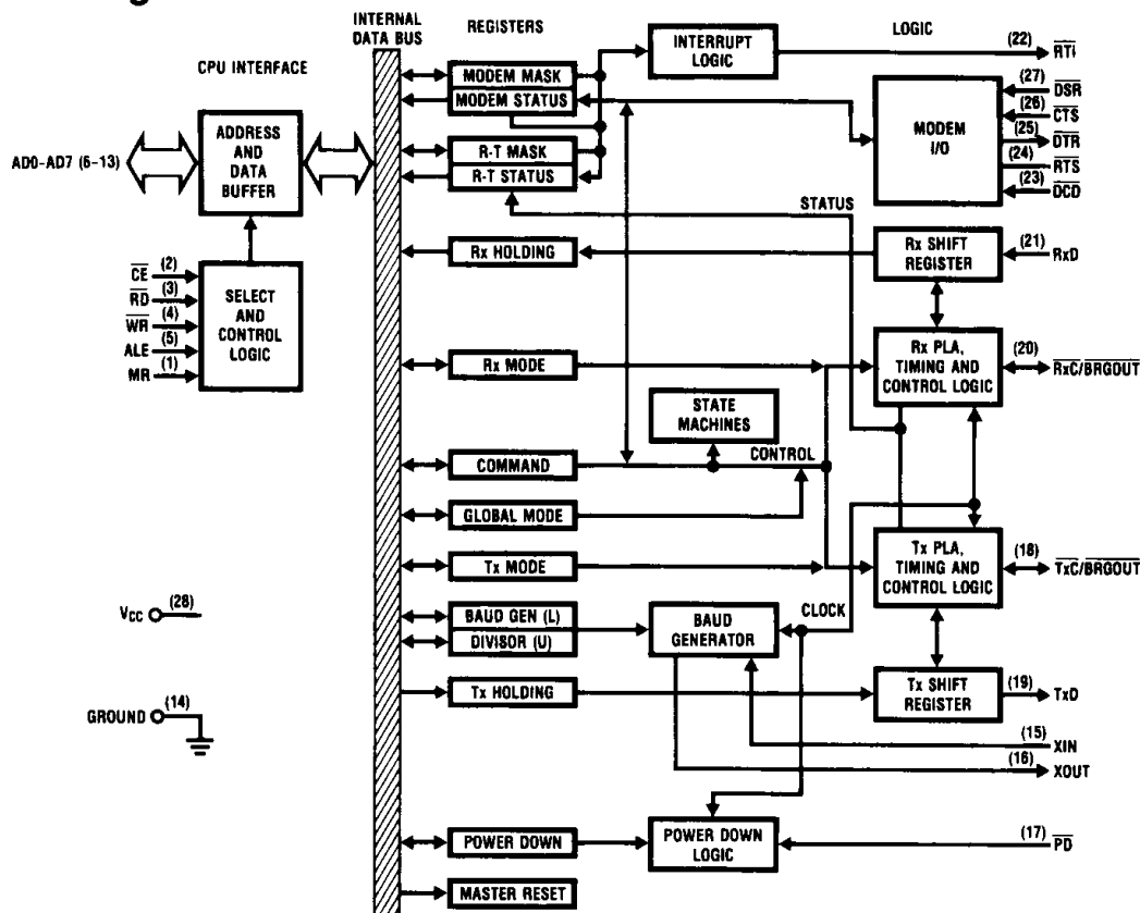
FIGURE 1. NSC858 Functional Block Diagram
