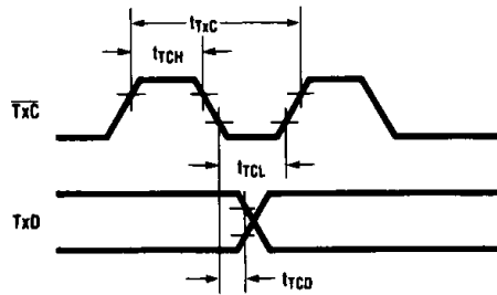
Transmitter Timing
