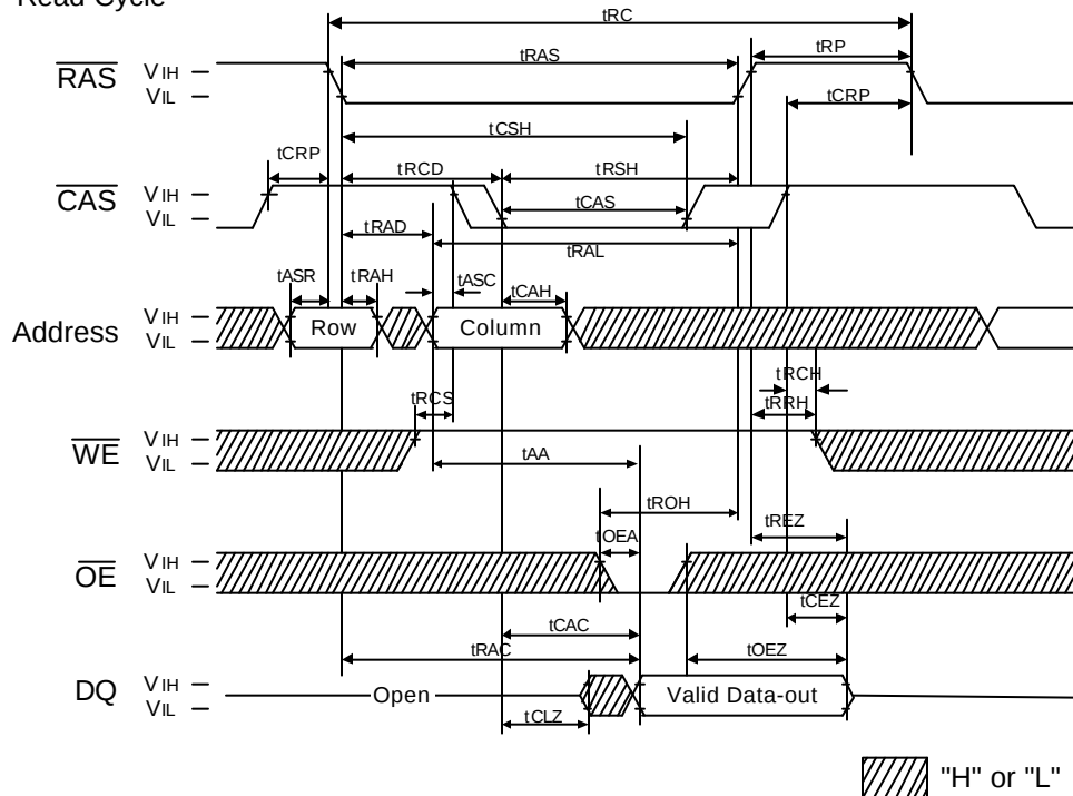
Read Cycle
