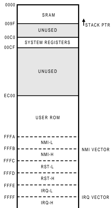
Figure 1.2. NT6880 Memory Map
