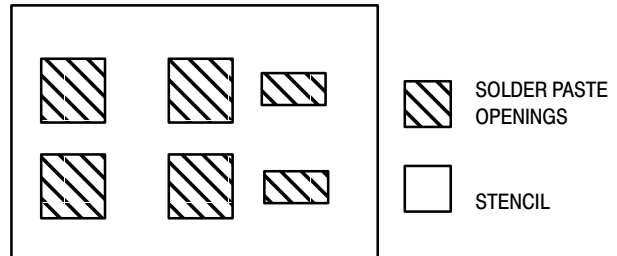
Figure 11. Typical Stencil for DPAK and D 2 PAK Packages
