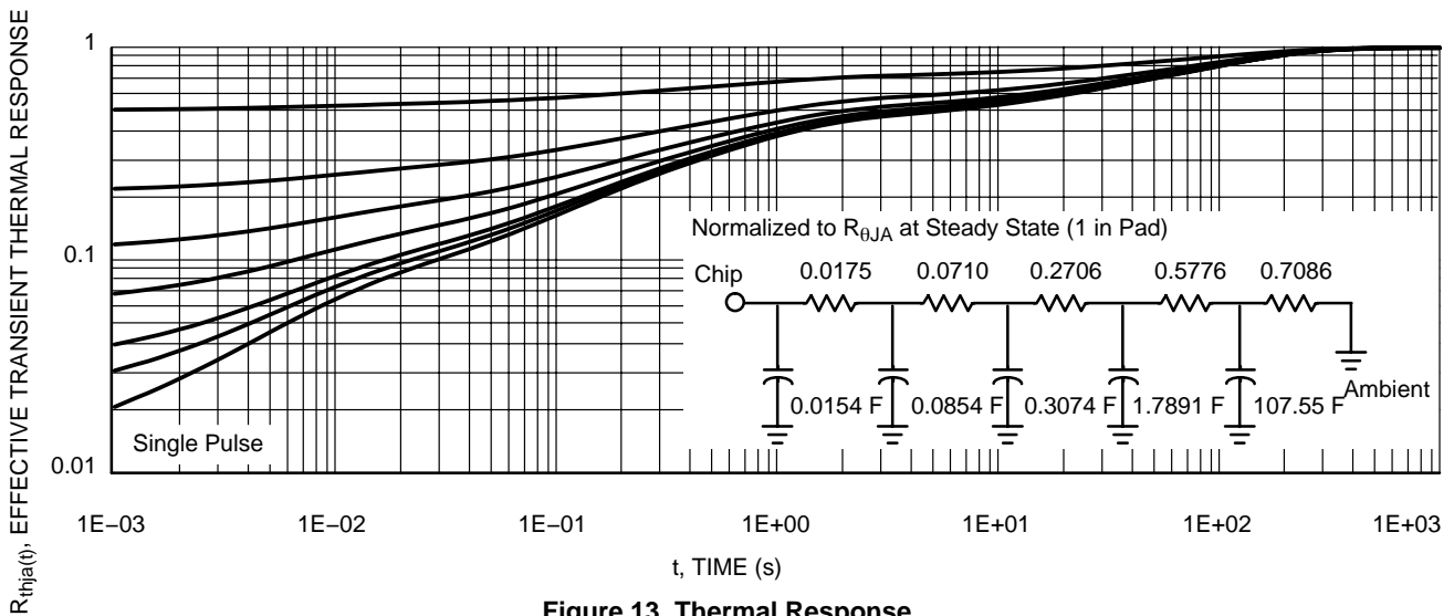
Figure 13. Thermal Response
