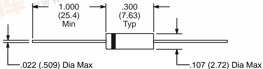
Color Band Denotes Cathode
