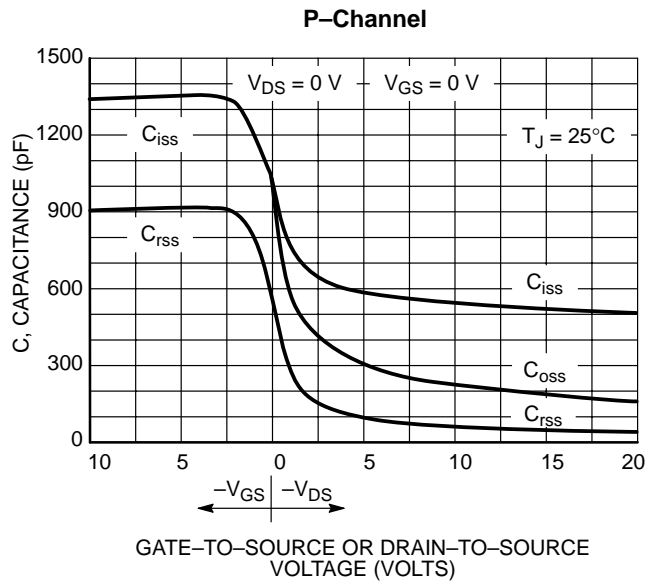
Figure 7. Capacitance Variation
