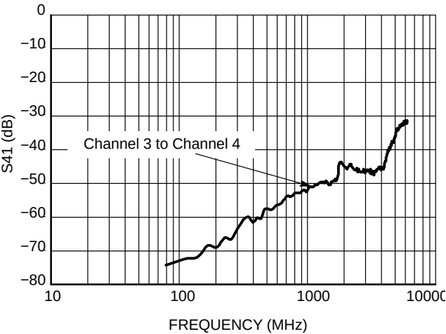
Figure 2. Analog Crosstalk Curve
